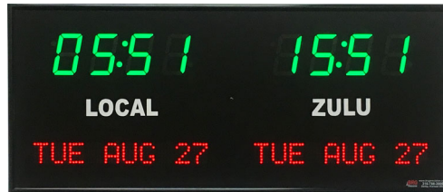
Model 6637H - 2.5" 4 digit bar segment LEDs for time, 1.2" 10 digit dot matrix LEDs for date, 1.0" white vinyl zone labels, 2 zones
