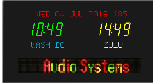
Model 6789X - 4.0" time, 2.0" zone labels, 2.0" 20 character date 4.0" dot matrix message display 36" wide, 2 zones
